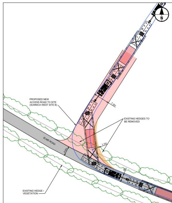
Figure 42: 1000T Crane Swept Path Analysis (Entry and Egress): Sunnica East Site B on Elms Road
