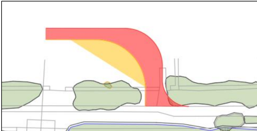
Figure 47 Figure 42 : Indicative Junction Layout: Option 2
